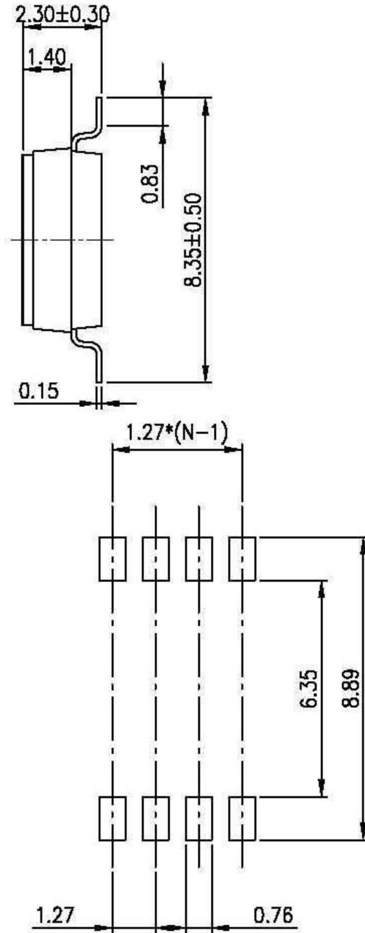
RECOMMENDED P.C.B. LAYOUT (TOP VIEW)
